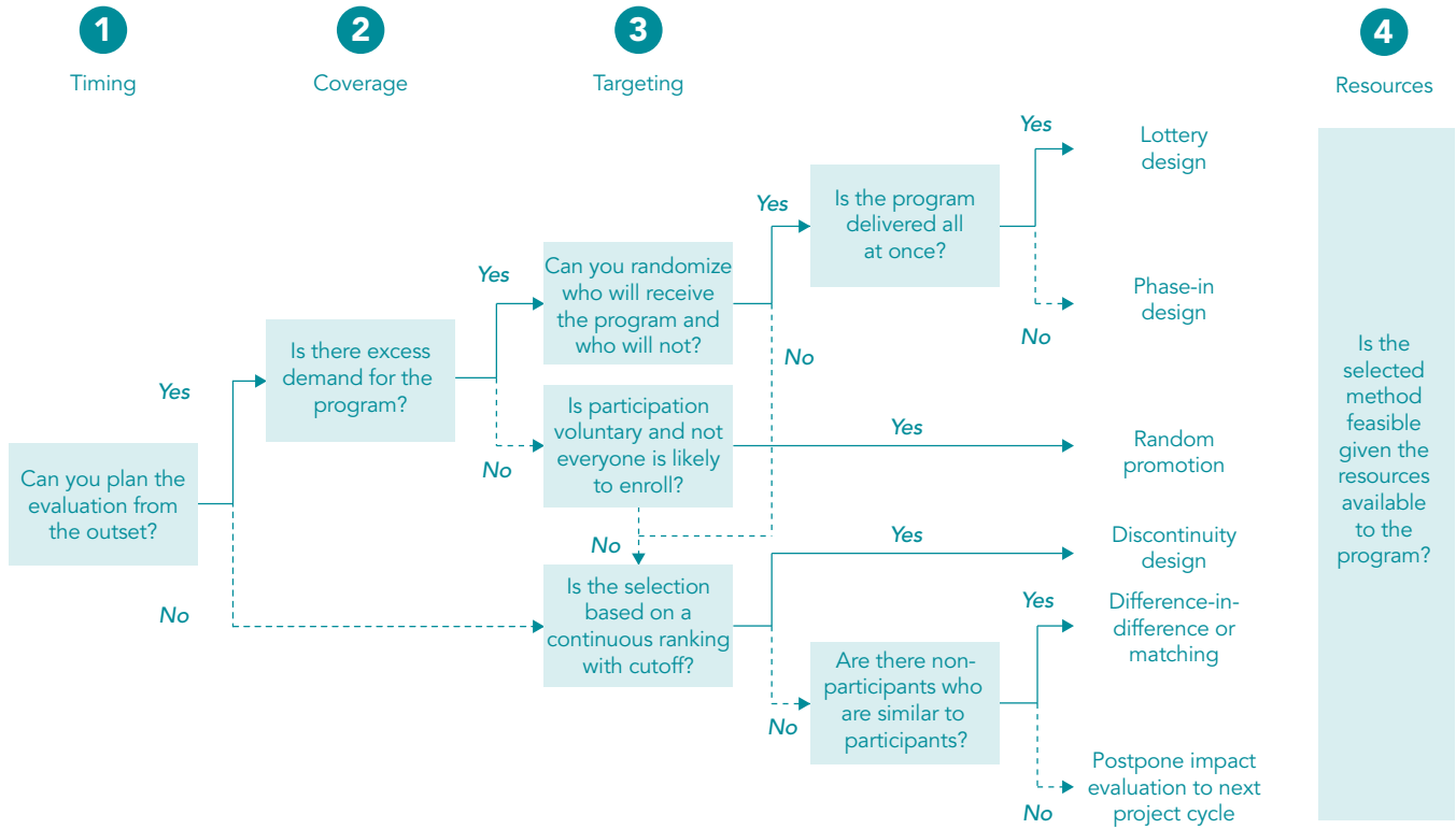
FIGURE 6.1 Decision tree for choosing impact evaluation techniques
